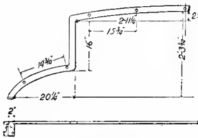
Figs. 1248-1249. Carline-plate (10).
